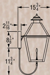
WALL MOUNT - SIDE
