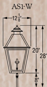
WALL MOUNT - FRONT
