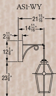
WALL YOKE MOUNT
